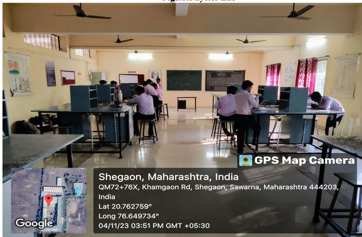
Fig 2.2:Chemistry Lab
